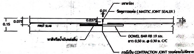
CONSTRUCTION JOINT AND CONTRACTION JOINT NOT TO SCALE
